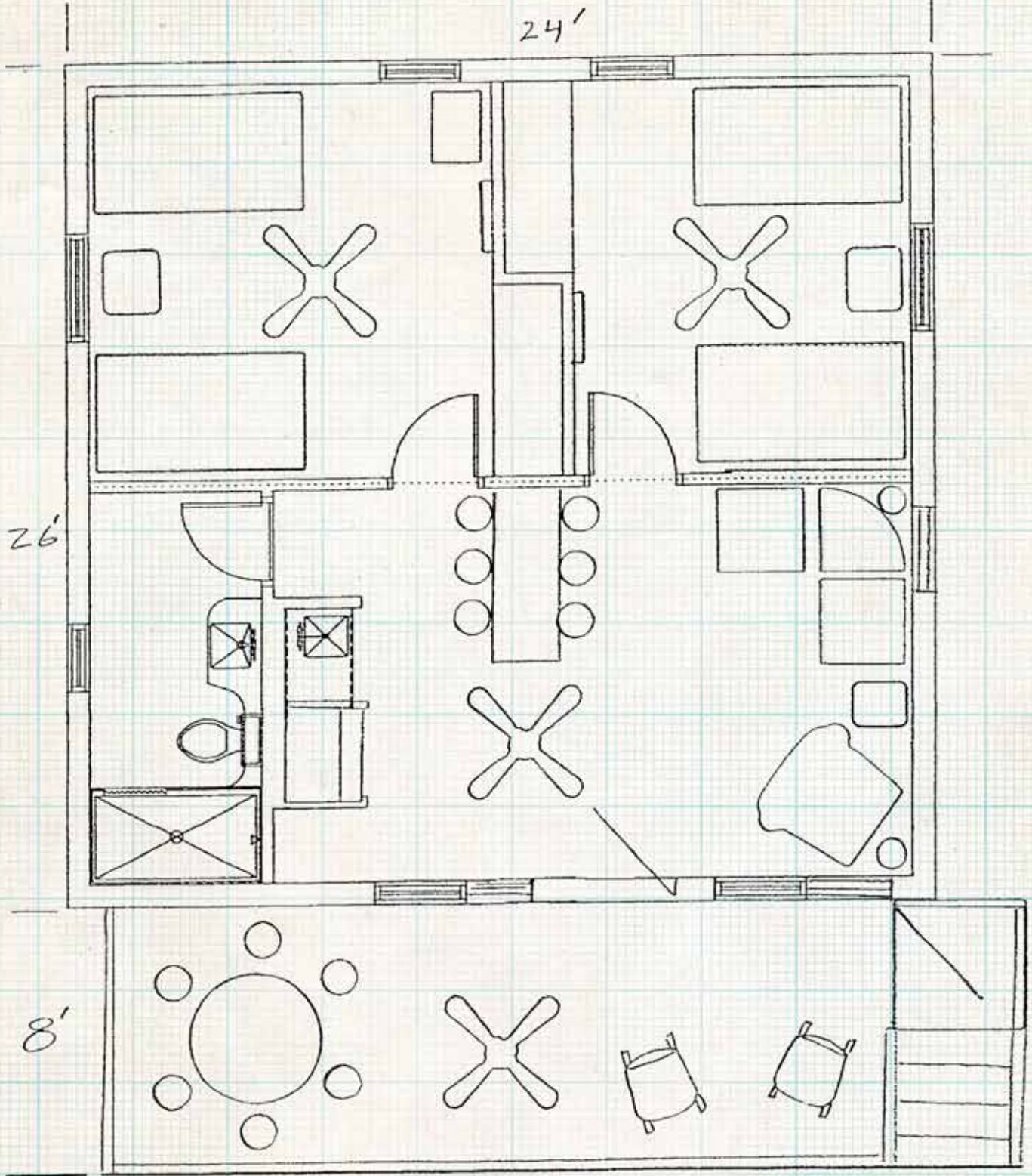
SNPJ Recreation Center Two Bedroom Upper Cabins Floor Plan Cabins #1 and #2
